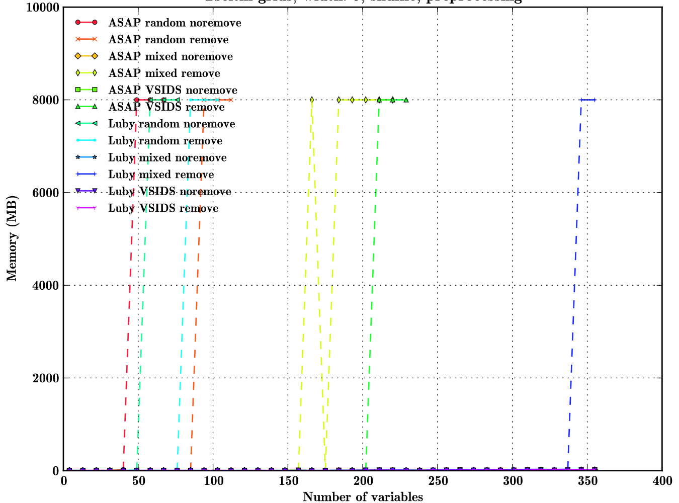
Tseitin grids, width: 5, shuffle, preprocessing
