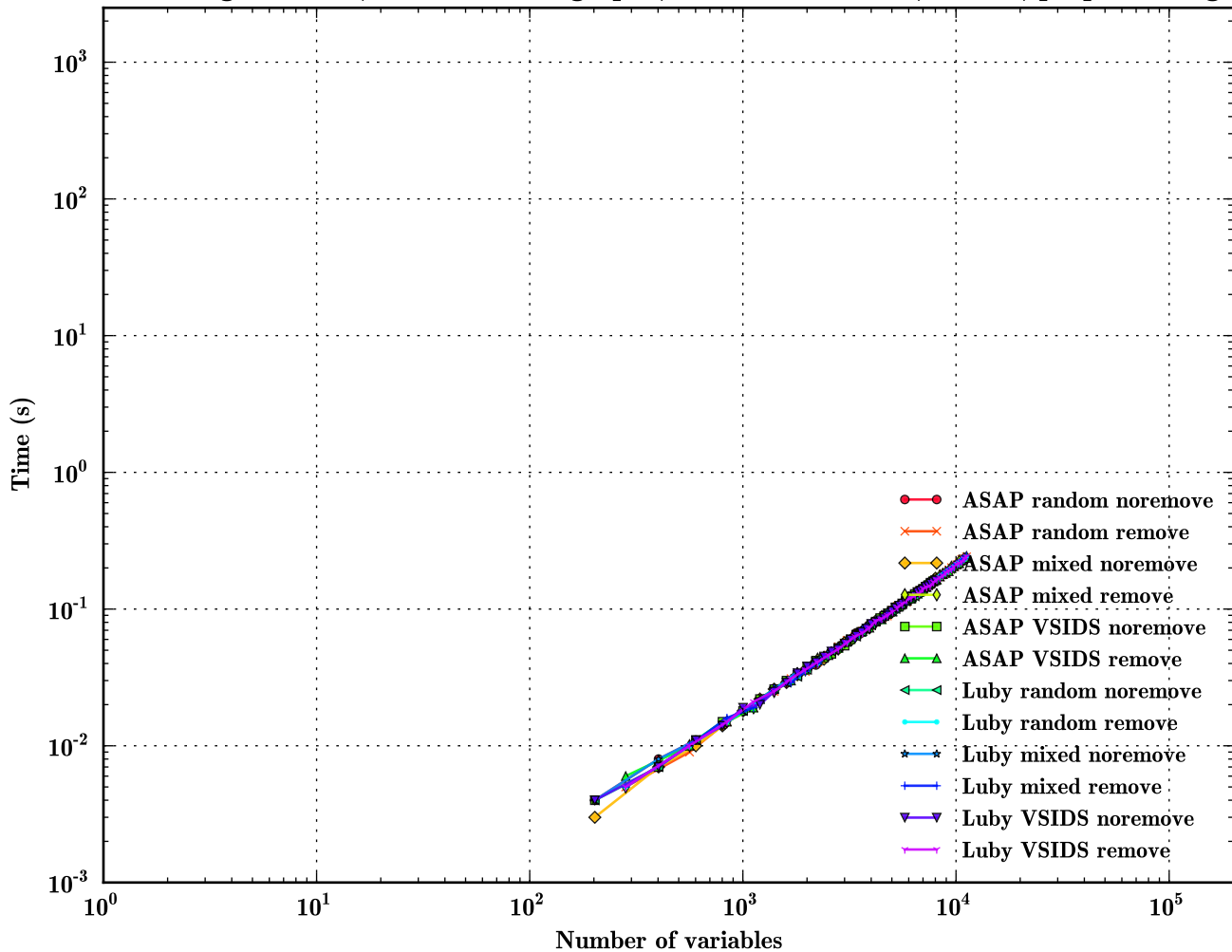
Pebbling formulas, width 2 chain graphs, substitution xor 2, shuffle, preprocessing
