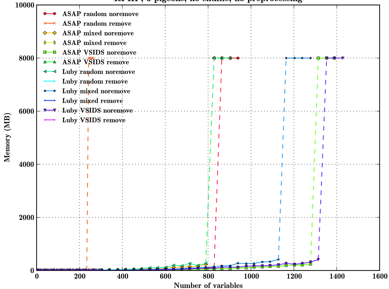
RPHP, 3 pigeons, no shuffle, no preprocessing
