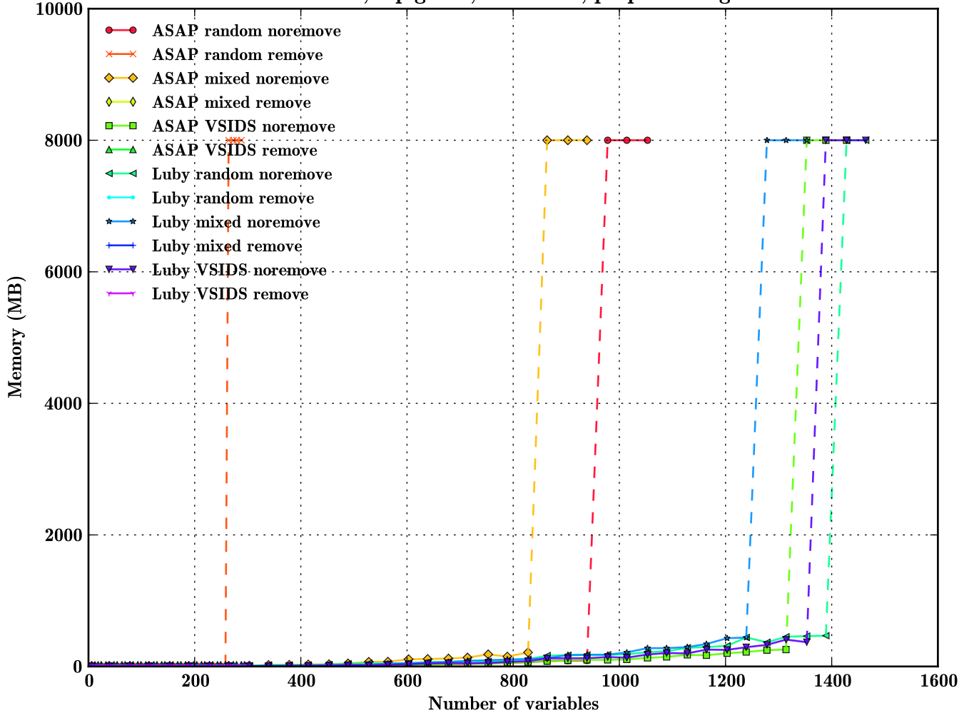
RPHP, 3 pigeons, no shuffle, preprocessing
