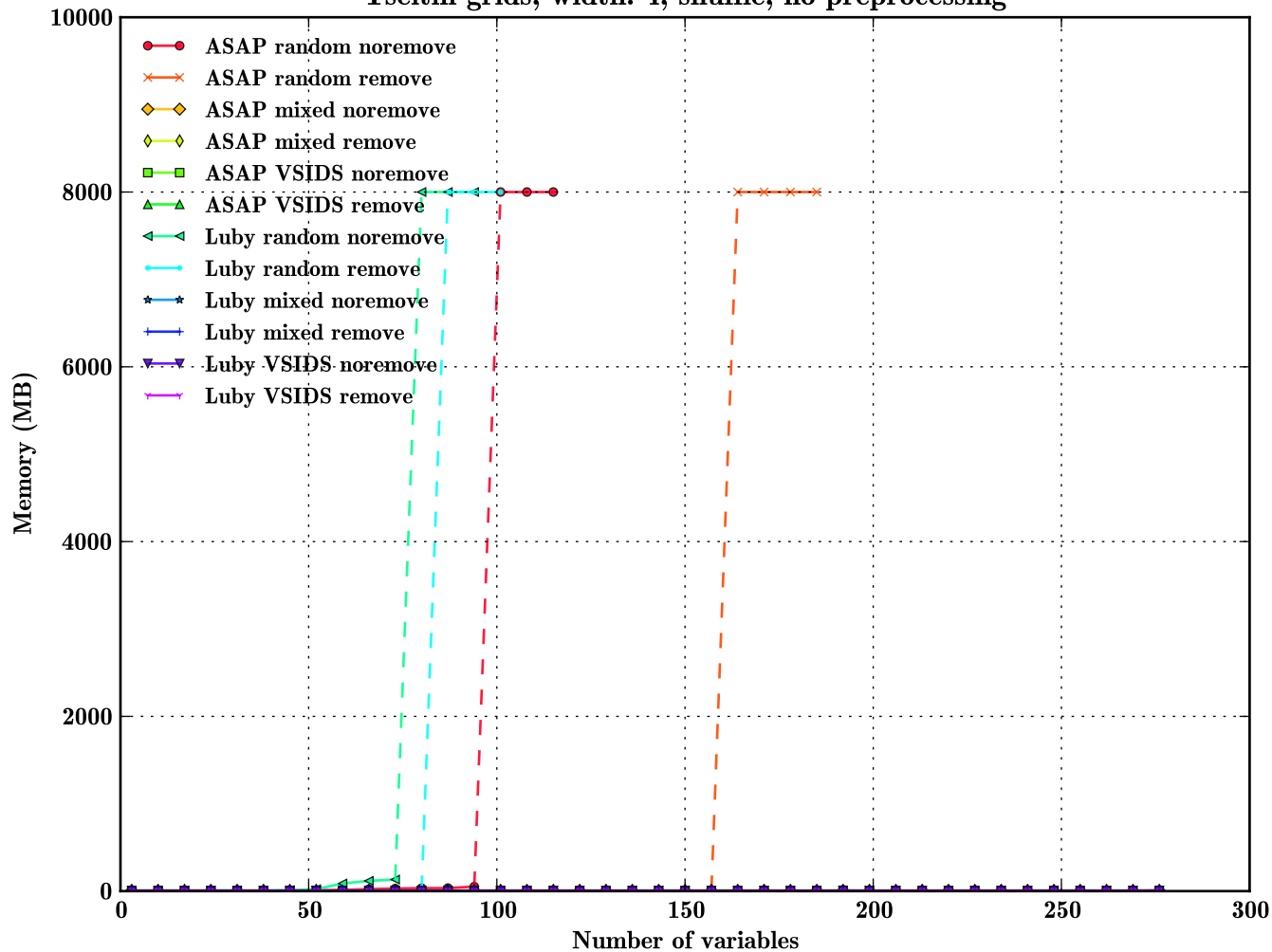
Tseitin grids, width: 4, shuffle, no preprocessing
