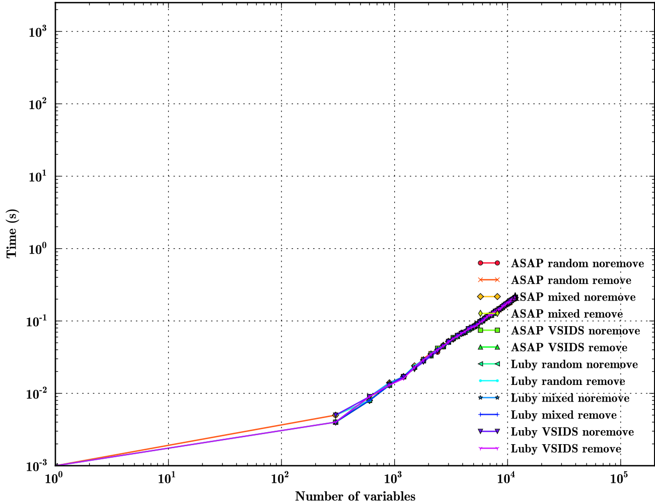
Tseitlin grids, width: 2, no shuffle, preprocessing
