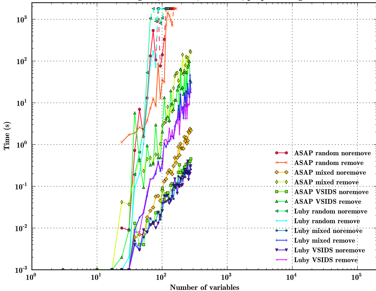
Tseitlin grids, width: 4, no shuffle, preprocessing
