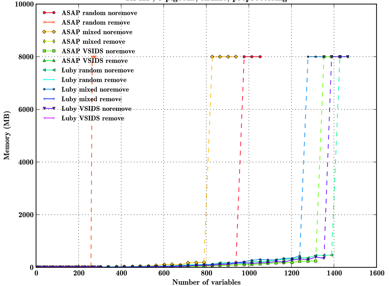
RPHP, 3 pigeons, shuffle, preprocessing
