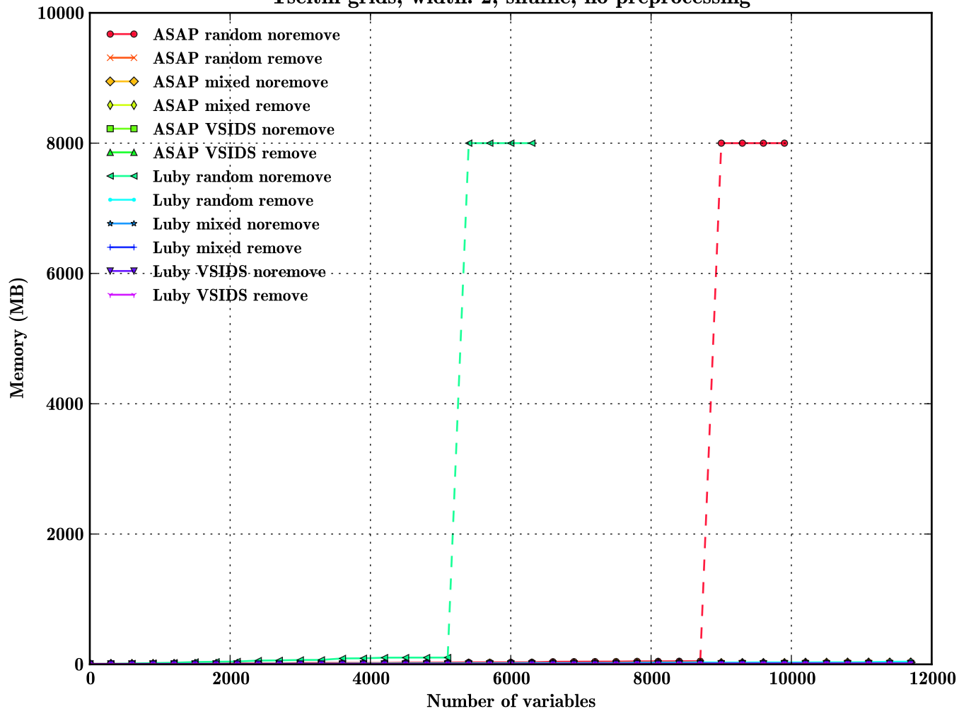
Tseitlin grids, width: 2, shuffle, no preprocessing
