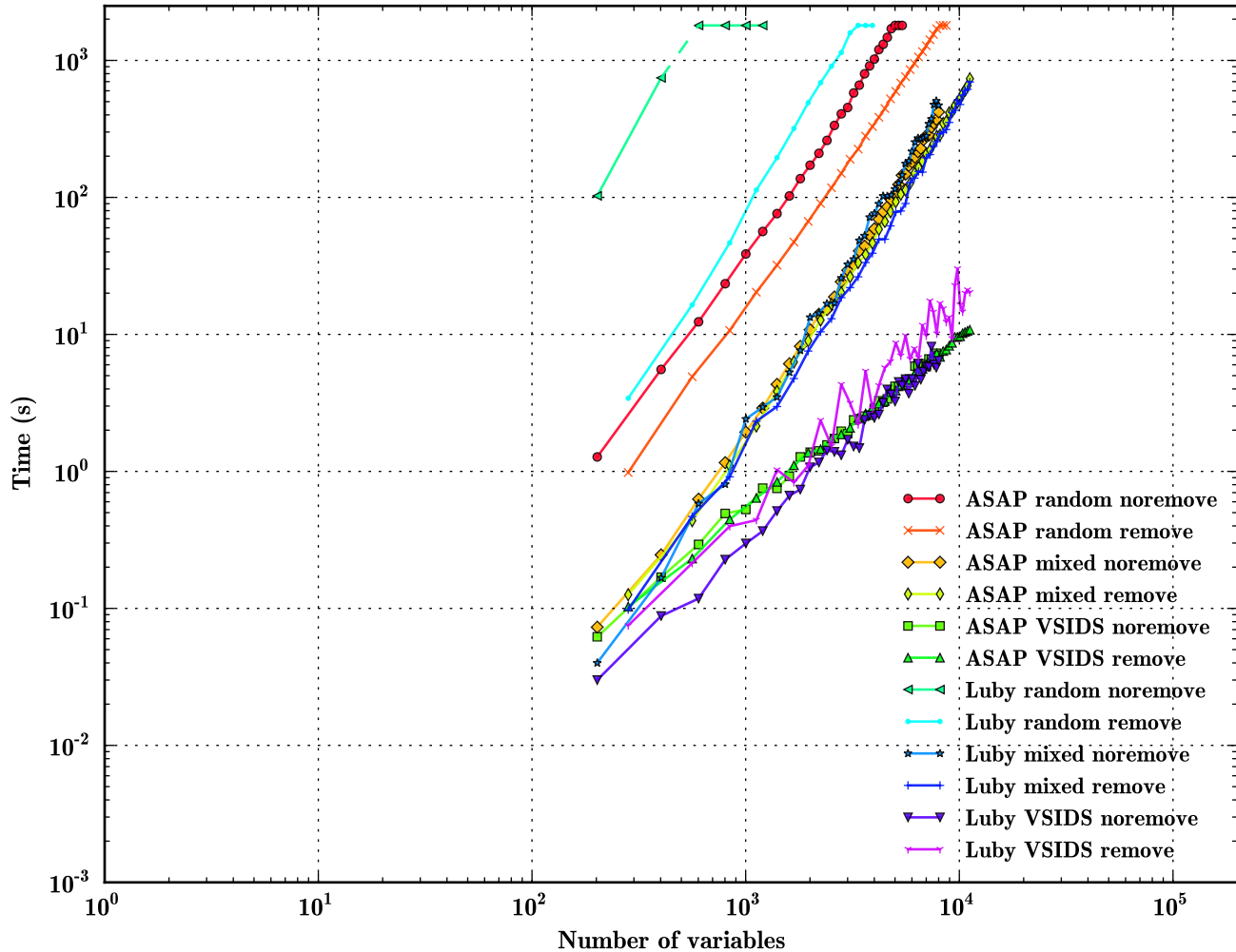
Pebbling formulas, width 2 chain graphs, substitution xor 2, shuffle, no preprocessing
