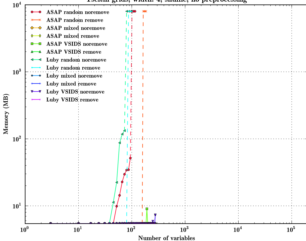
Tseitlin grids, width: 4, shuffle, no preprocessing
