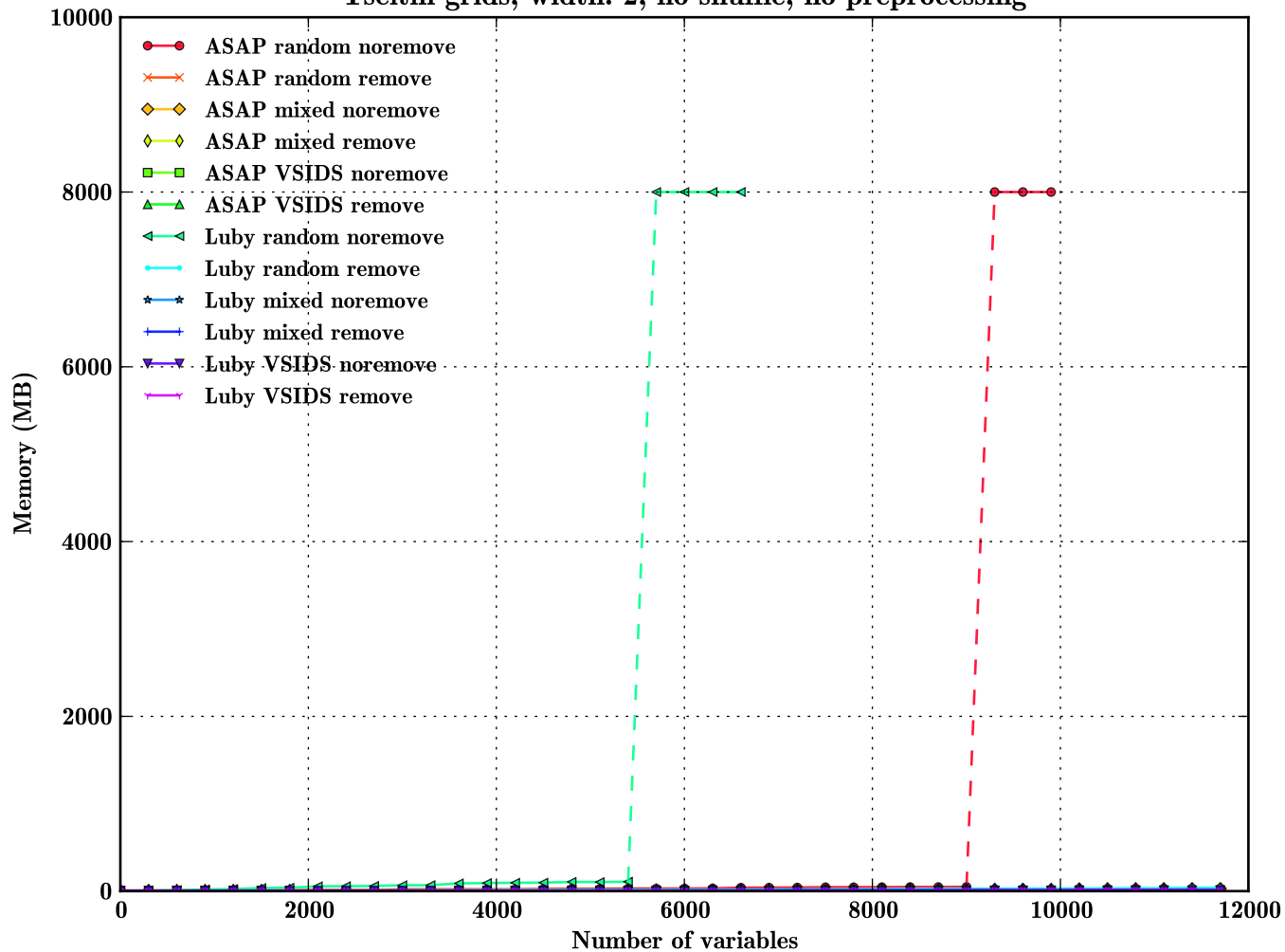
Tseitin grids, width: 2, no shuffle, no preprocessing
